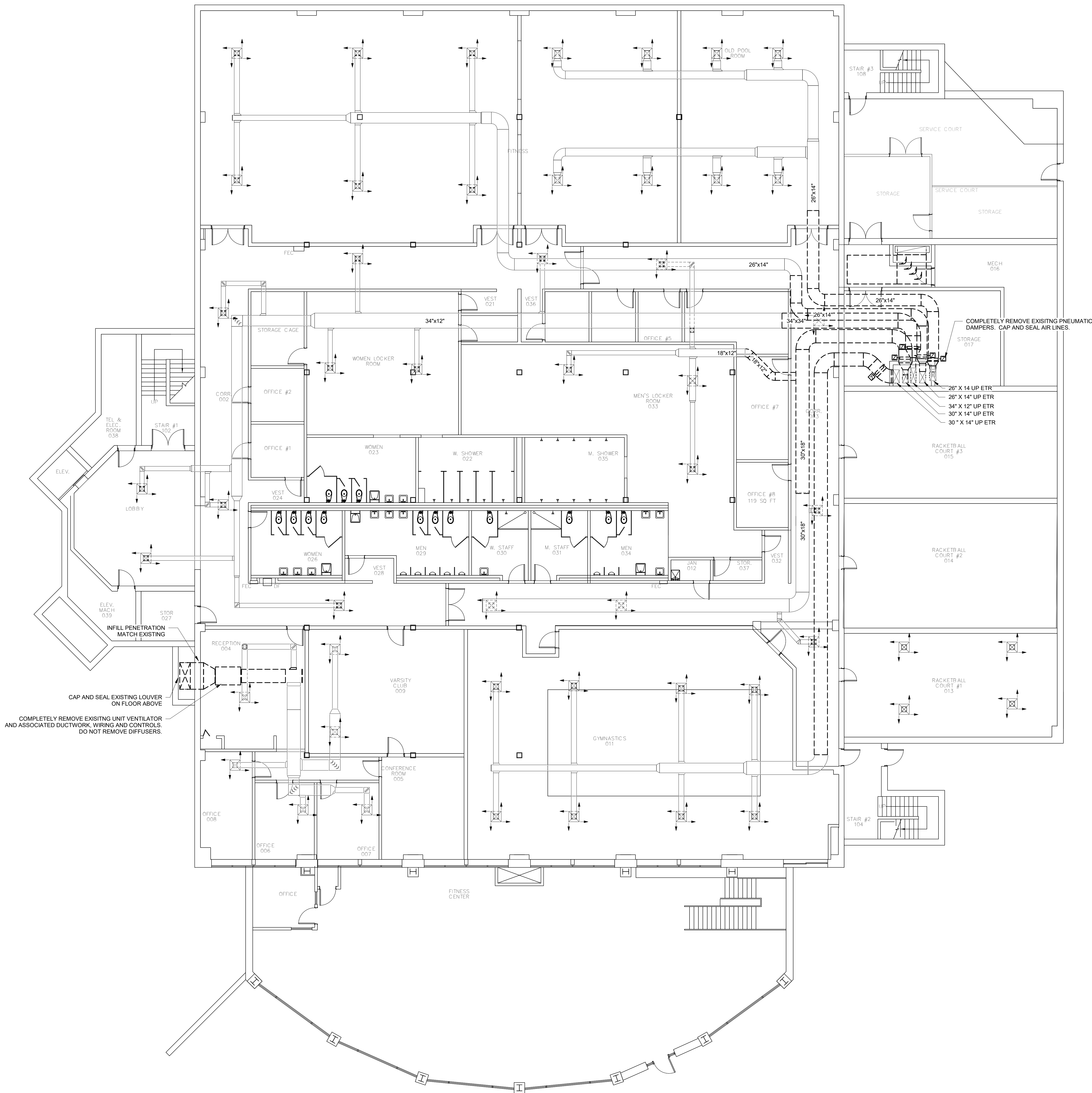
1 MECHANICAL DEMOLITION - LOWER LEVEL SCALE: 1/8" = 1'-0"
